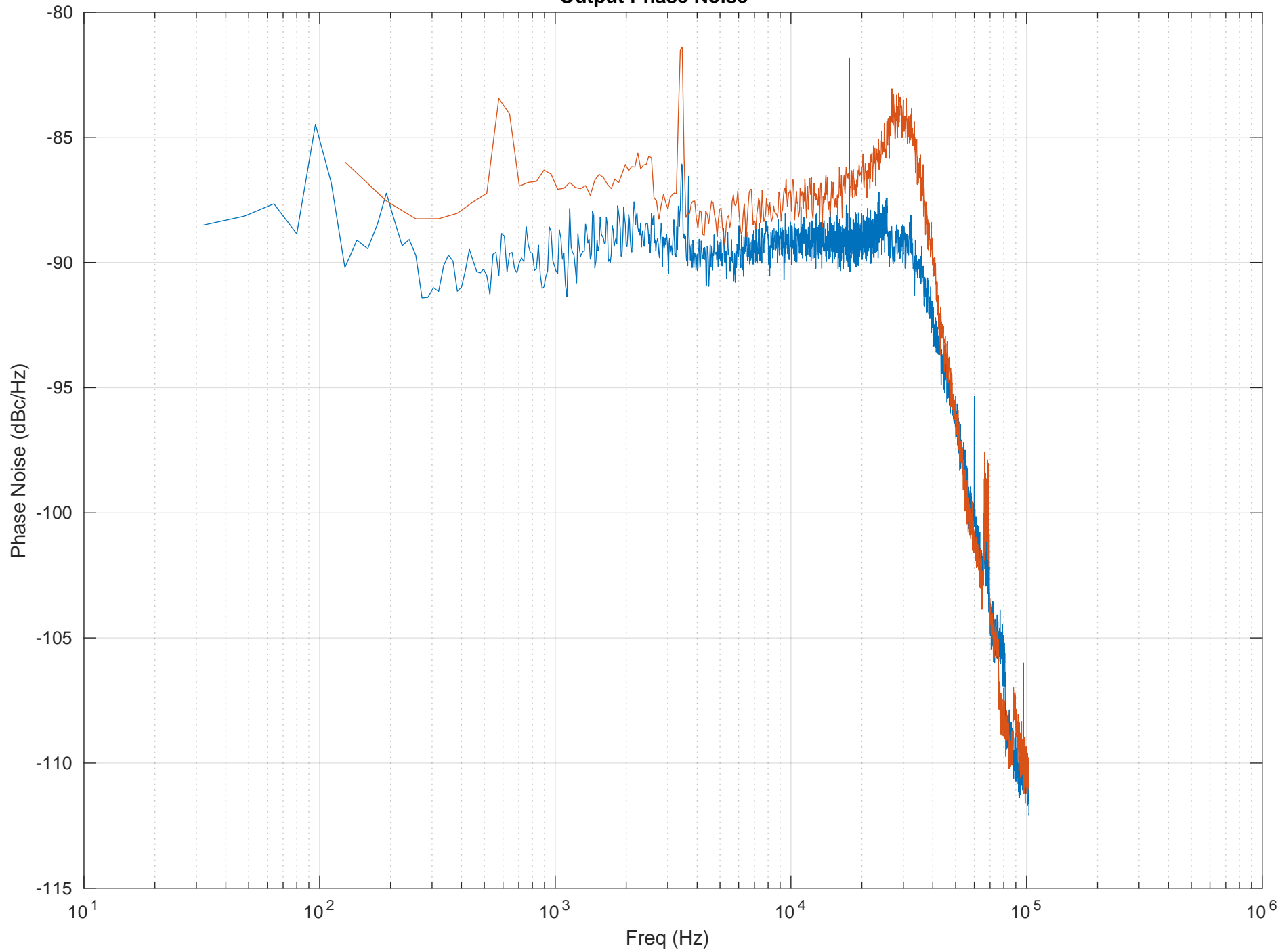
Output Phase Noise
