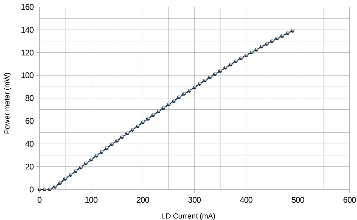
Optical Power vs LD Current
