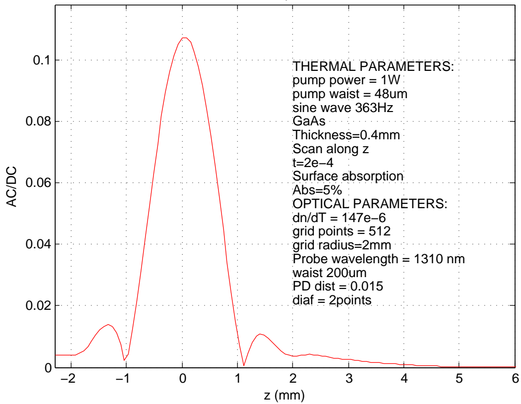
Surface absorption of GaAs
