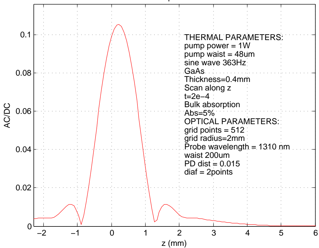
Bulk absorption of GaAs
