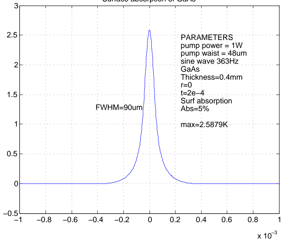
Surface absorption of GaAs
